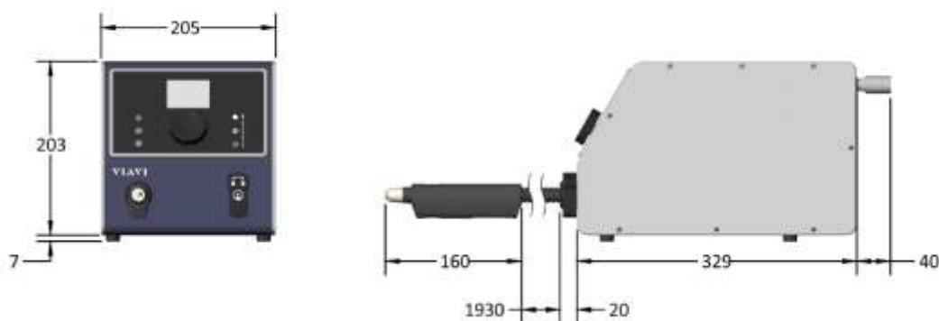
Figure 5: CleanBlastPRO dimensions
