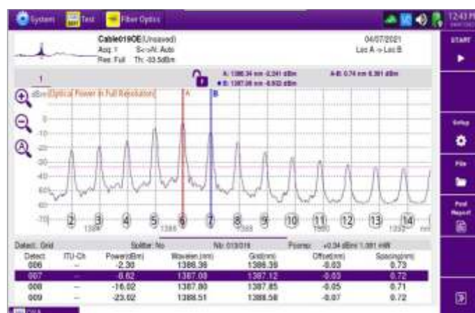
Optical Spectrum Analysis
