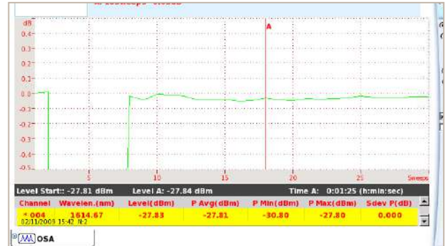
Drift power measurement
