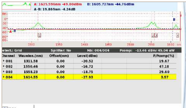
Spectral measurement displays trace and table
